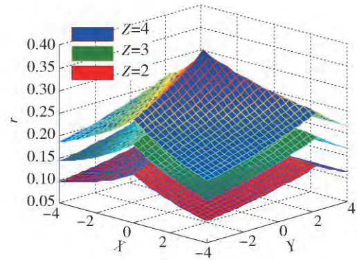
图 8 \beta_b = 90^\circ, \beta_m = 45^\circ 时 r 随位置参数变化 Fig. 8 r versus position parameters for \beta_b = 90^\circ and \beta_m = 45^\circ
