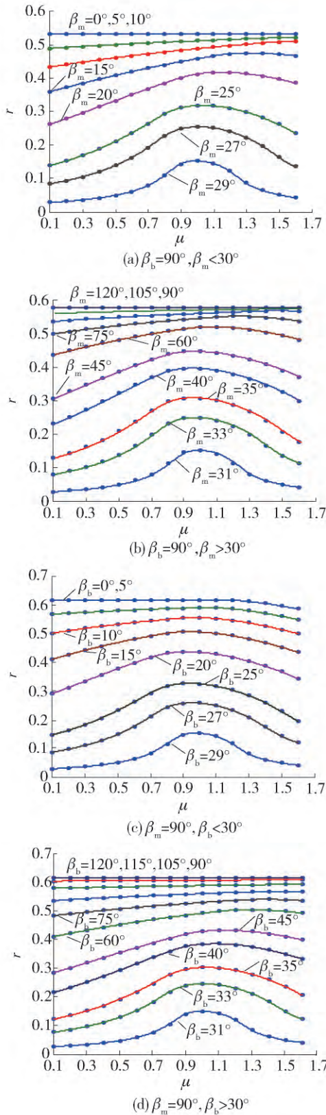
图 7 位置 (0, 0, 4) \beta_m, \beta_b 给定时 r 随 \mu 变化情况 Fig. 7 r versus \mu for constant \beta_m and constant \beta_b at position (0, 0, 4)
